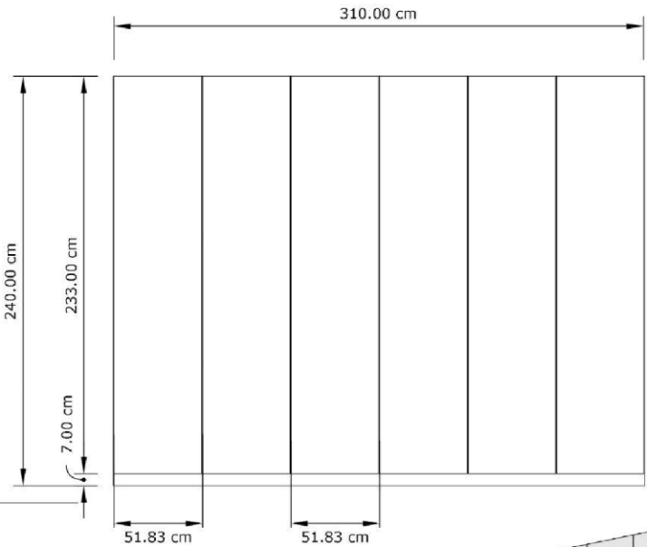
0 Front view
