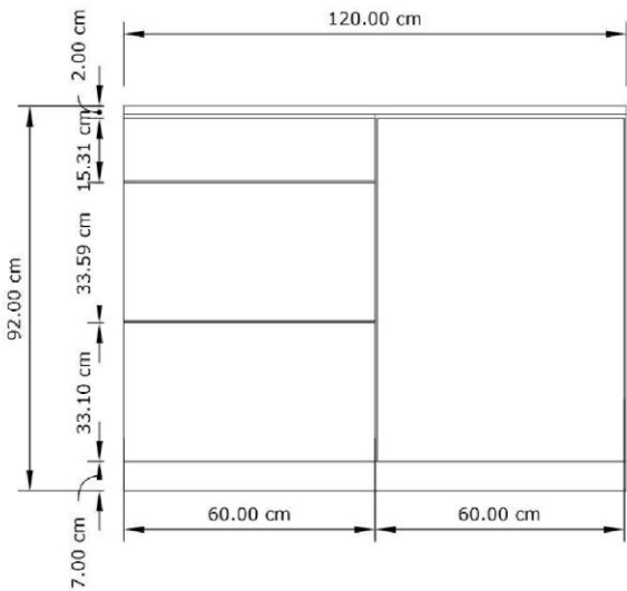
0 Front view Scale: 0" : 0"
