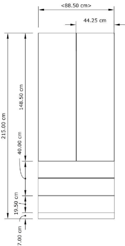
0 Front view Scale: 0" : 0"
