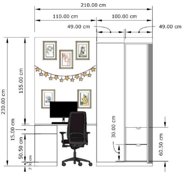
0 Front view
