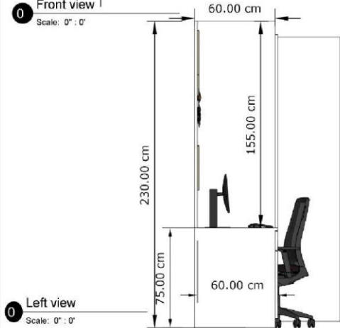
0 Front view
