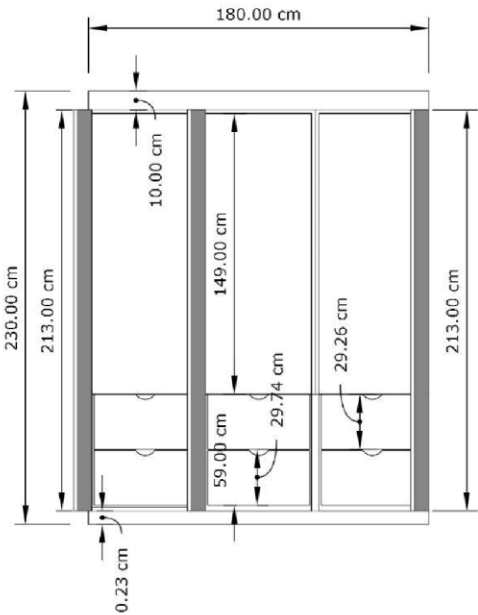
0 Front view
